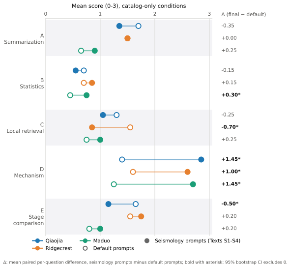
FIGURE 3. Per-category benchmark scores under default prompts (open circles) and after the Section V prompt-engineering scheme (filled circles), catalog-only condition. Connectors join the before and after values; the right column ( \Delta ) gives the mean paired per-question change, final minus default, with an asterisk where the 95% bootstrap interval excludes zero. Physical-mechanism questions (Category D) improve most; precise-statistics questions (Category B) remain architecture-limited.
