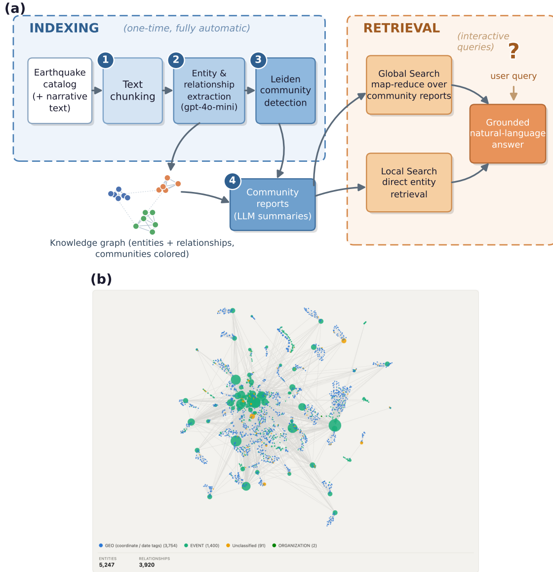
FIGURE 2. (a) Schematic of the GraphRAG indexing and retrieval pipeline. (b) Entity-relationship graph automatically constructed by GraphRAG from the Qiaojia catalog (5,247 entities; 3,920 relationships), with no hand-designed schema; GEO (coordinate/date tags), EVENT (individual earthquake records), and a small residual of Unclassified/Organization entities from generic extraction.
